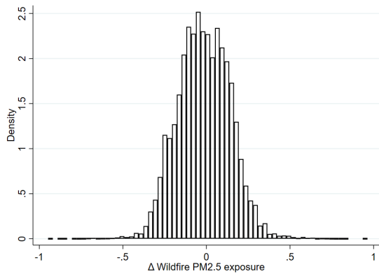
Yearly wildfire PM 2.5 exposure
