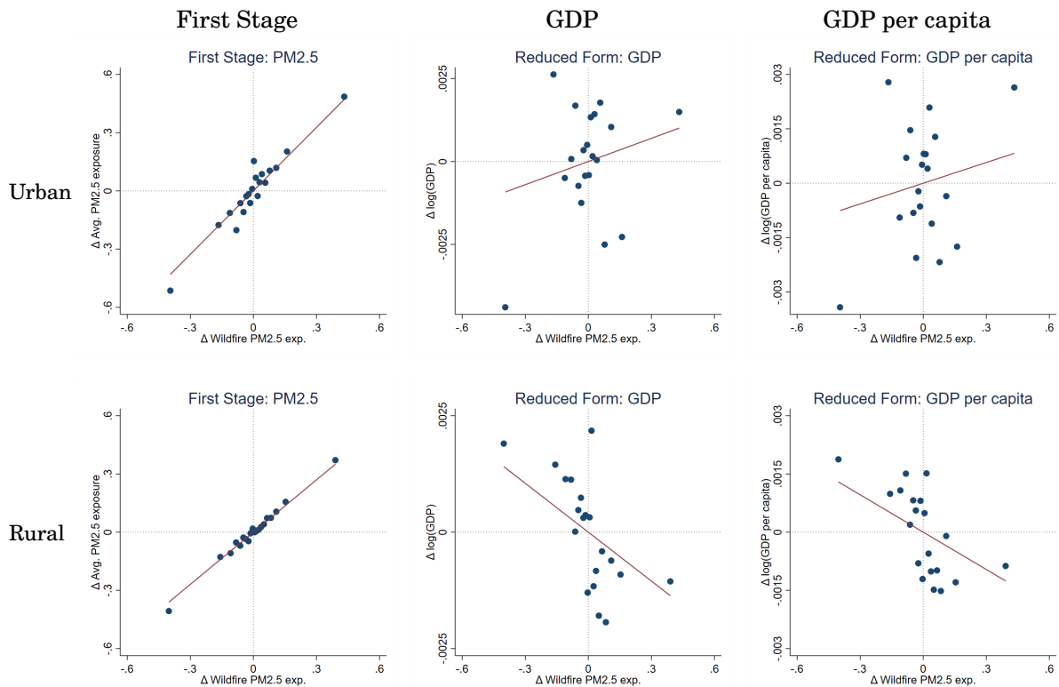
Figure B4: Binscatters of the first stage and reduced form for urban and rural counties reported in Table 5. Each dot represents a 5% of the counties, population-weighted. Outcomes and PM_{2.5} exposure are cleaned of all influence of fixed effects and control variables.
