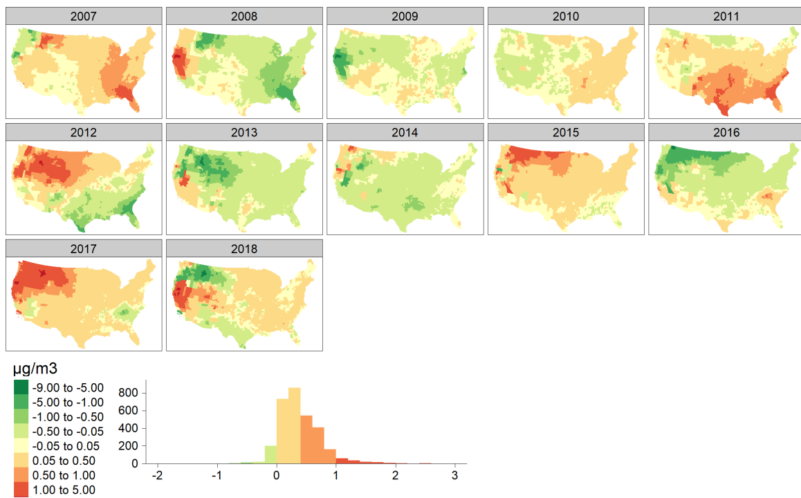
Figure B2: Geographical distribution of yearly changes of exposure to Wildfire PM 2.5
