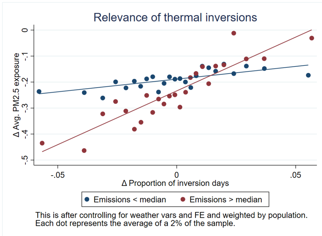
Figure A1: Descriptive relation between changes in the proportion of thermal inversions in a year and the average exposure to PM 2.5 .
