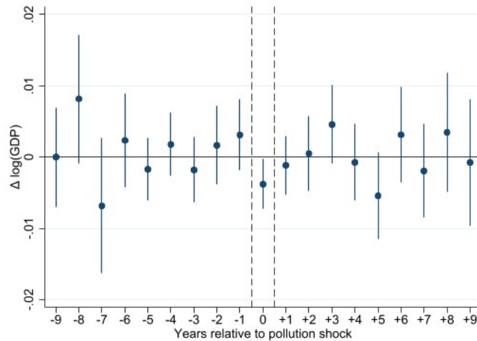
Figure B6: Estimated coefficients of \beta_1 For the effect of \Delta PM_{2.5,t=0} on \Delta \log(GDP_t) for 9 years before and after in rural areas with 95% C.I.. t = 0 corresponds with the effect in rural areas from Table 5.
