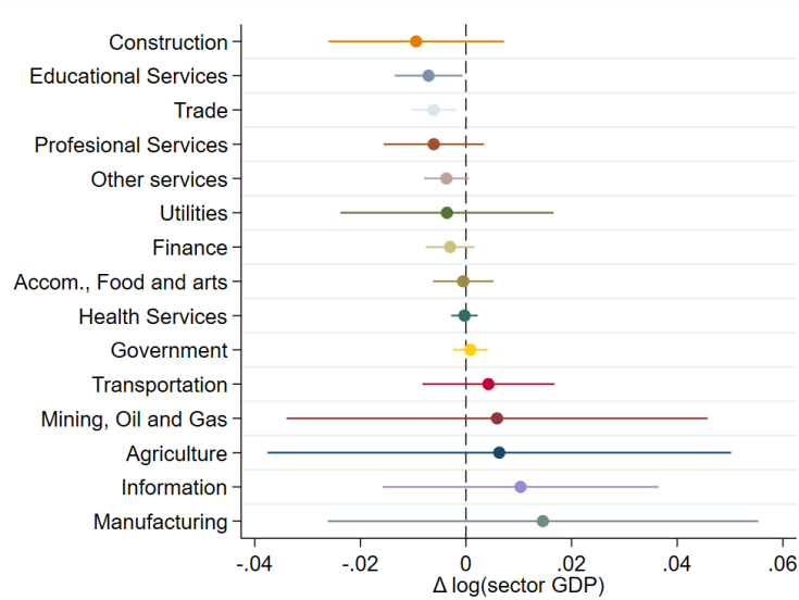
Figure B5: Summary of the impact of an 1\mu\text{g} increase in \text{PM}_{2.5} on sector-level GDP with 95% CI. Full results are available in Table B.1, in the Appendix. Not corrected for multiple hypothesis.
