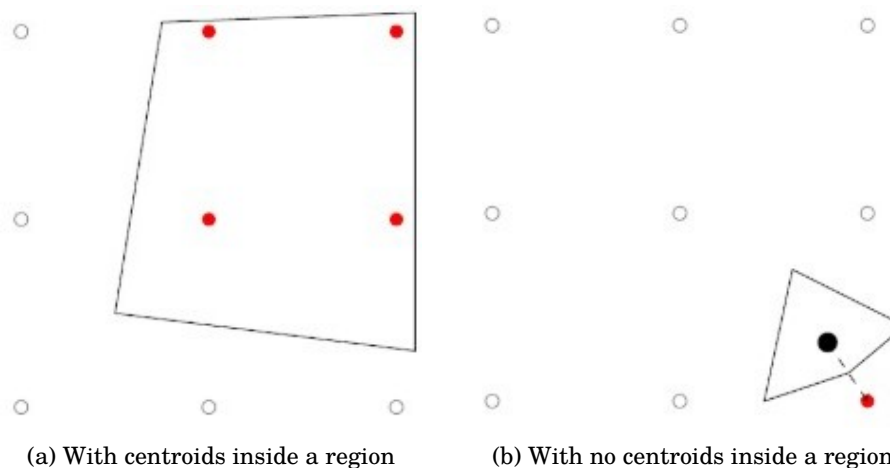
Figure B11: Imputation of raster values to counties (image from Dechezleprêtre et al. (2019) )
