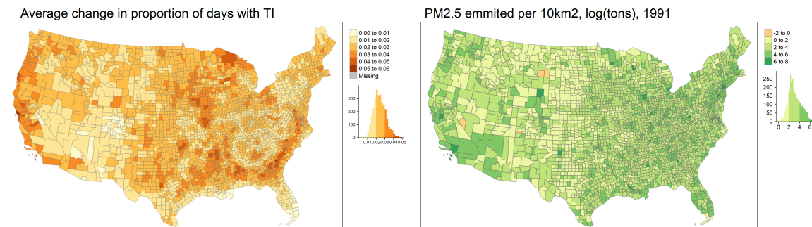
Figure A2: Identifying variation of the thermal inversion instrument.
